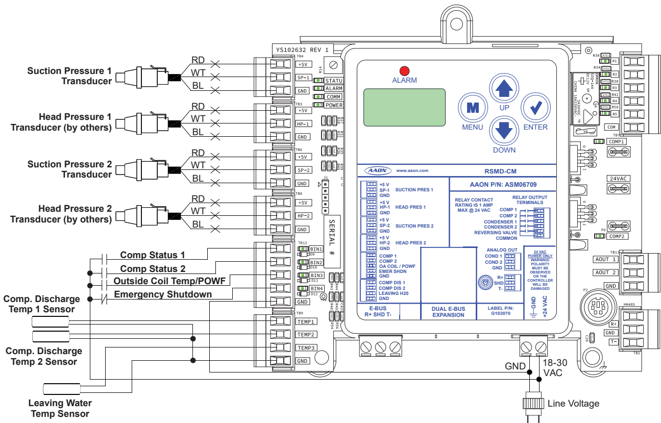
Figure 2: RSMD-CM Inputs Wiring
