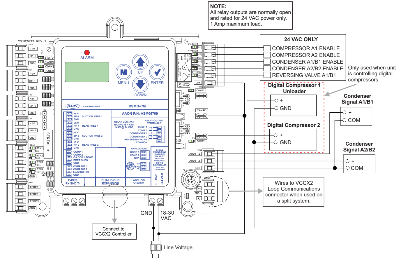
Figure 14: A1/B1 Wiring
