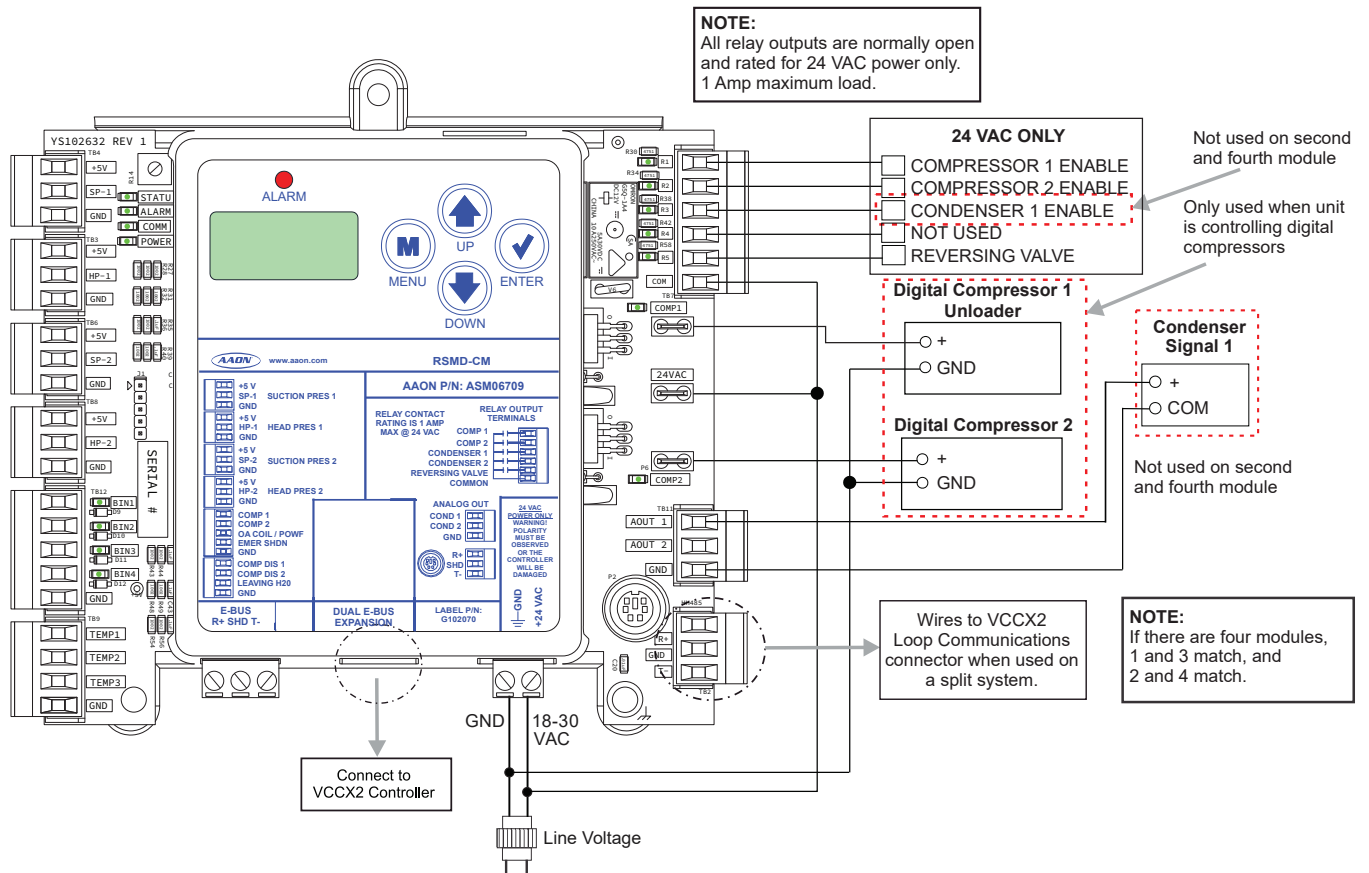
Figure 10: Single Condenser Per Two Modules
