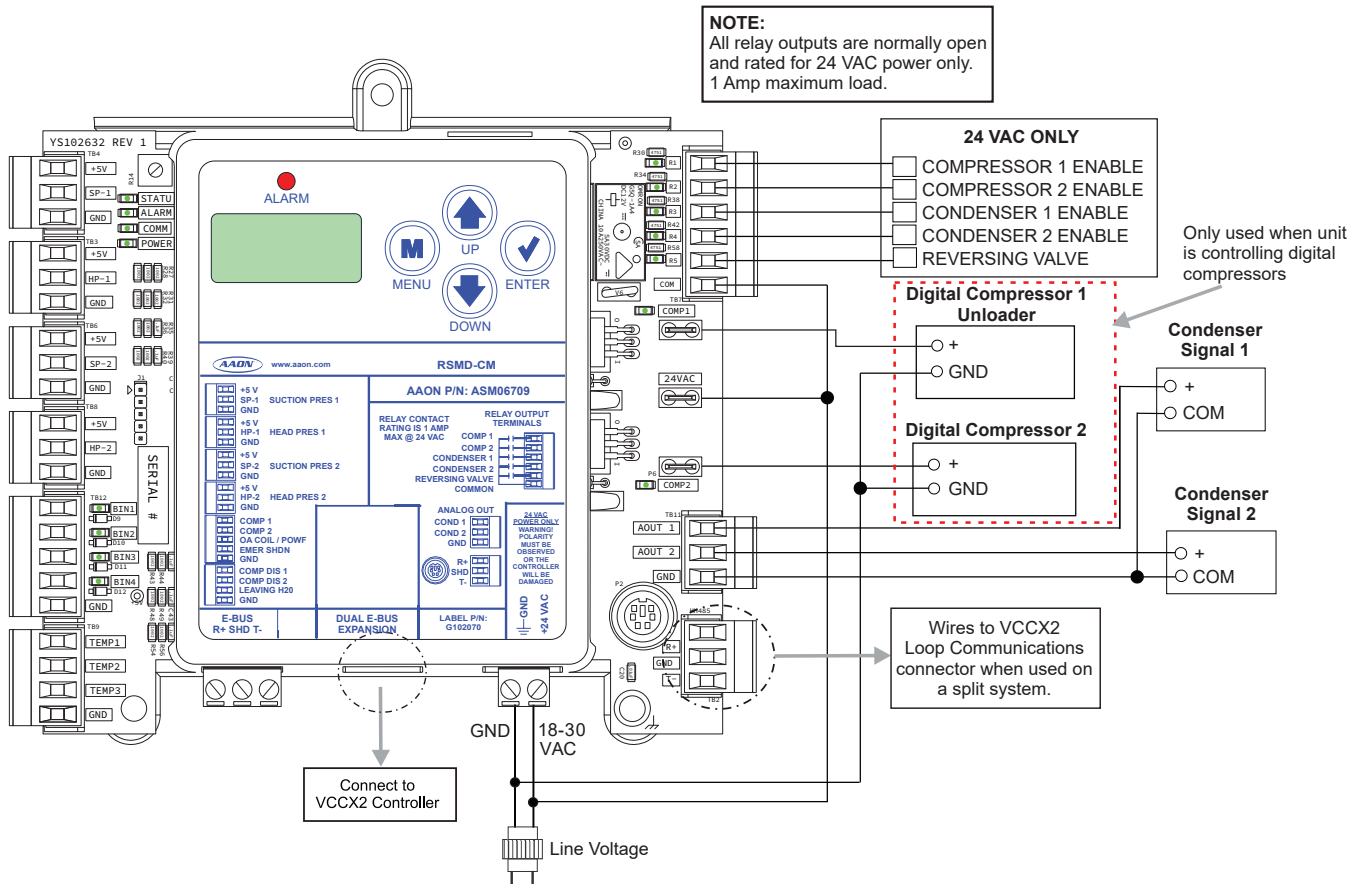
Figure 8: Single Condenser Per Module
