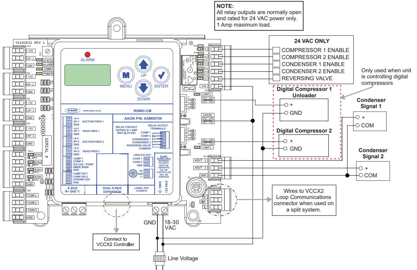
Figure 6: Two Condenser Operation (Default)
