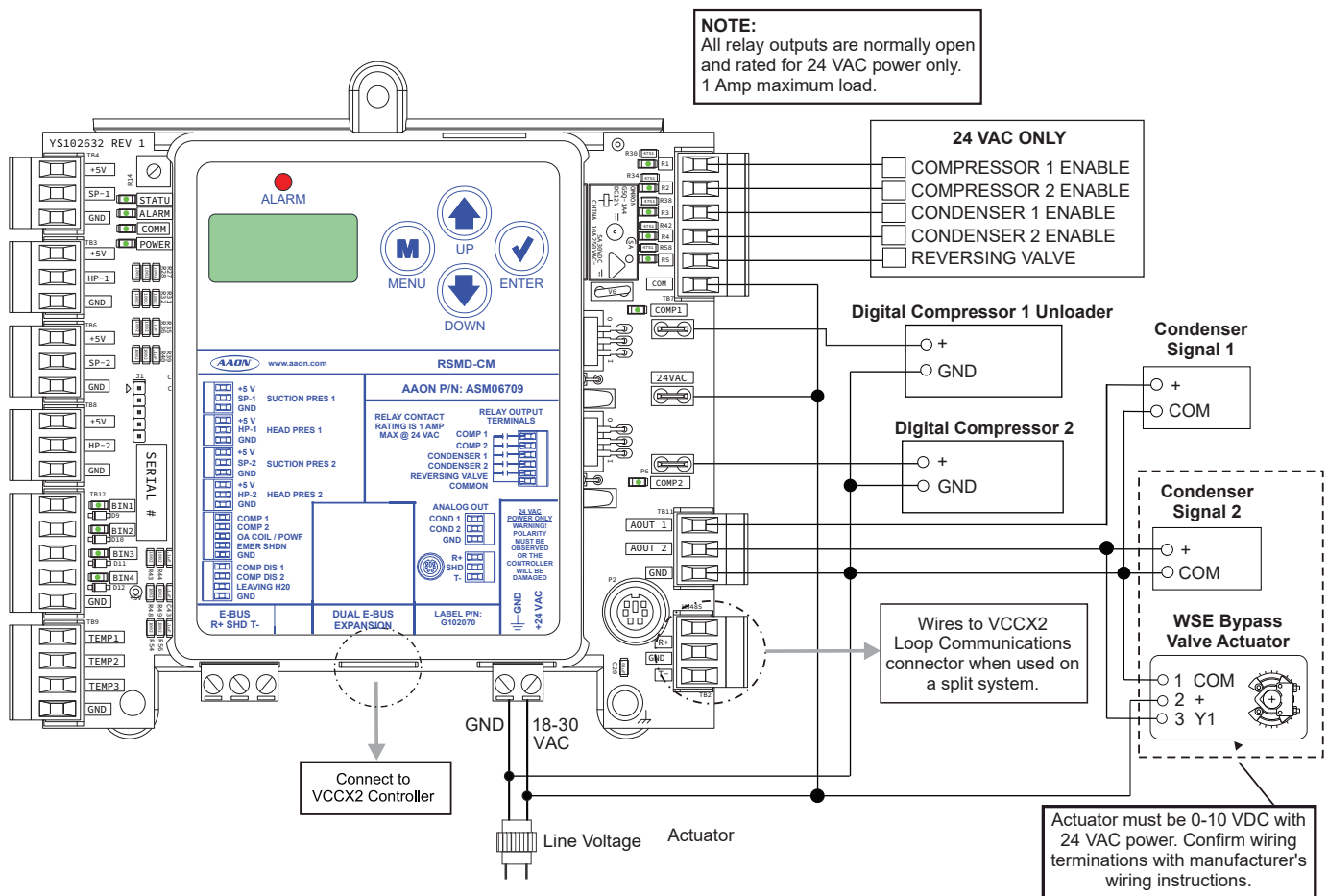
Figure 3: RSMD-CM Outputs Wiring
