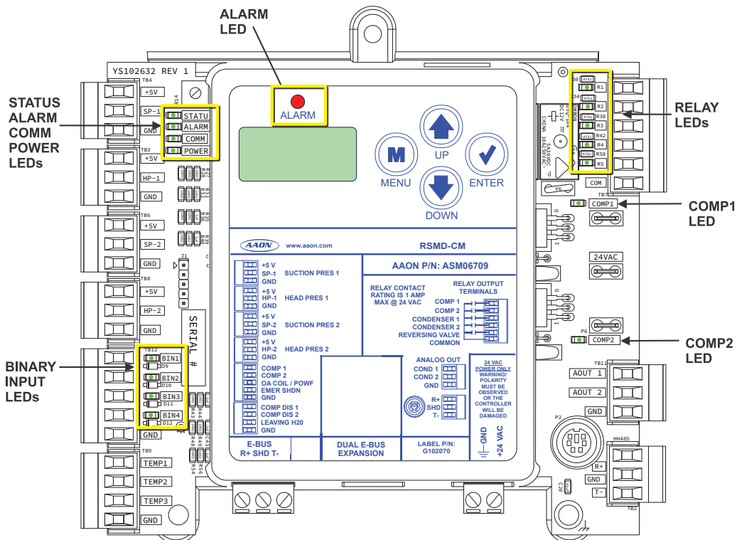
Figure 5: RSMD-CM LED Locations
