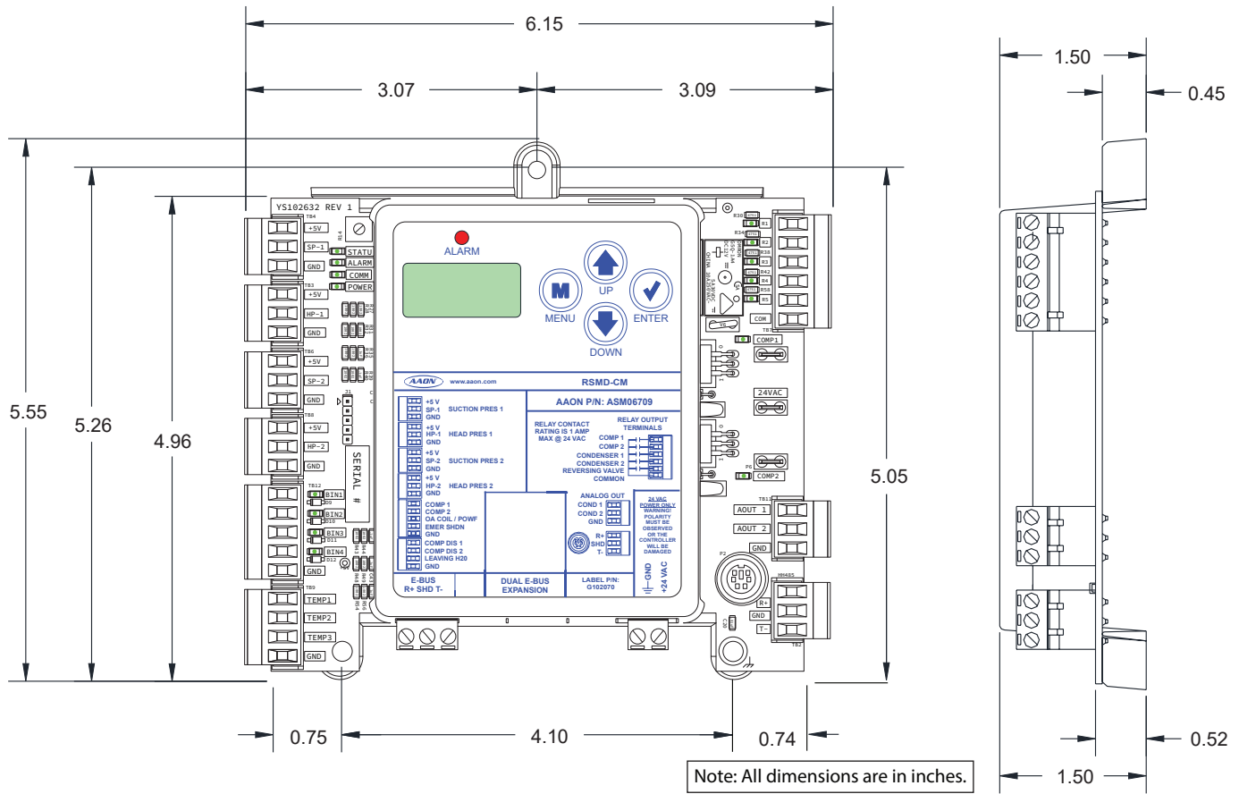
Figure 1: RSMD-CM Dimensions
