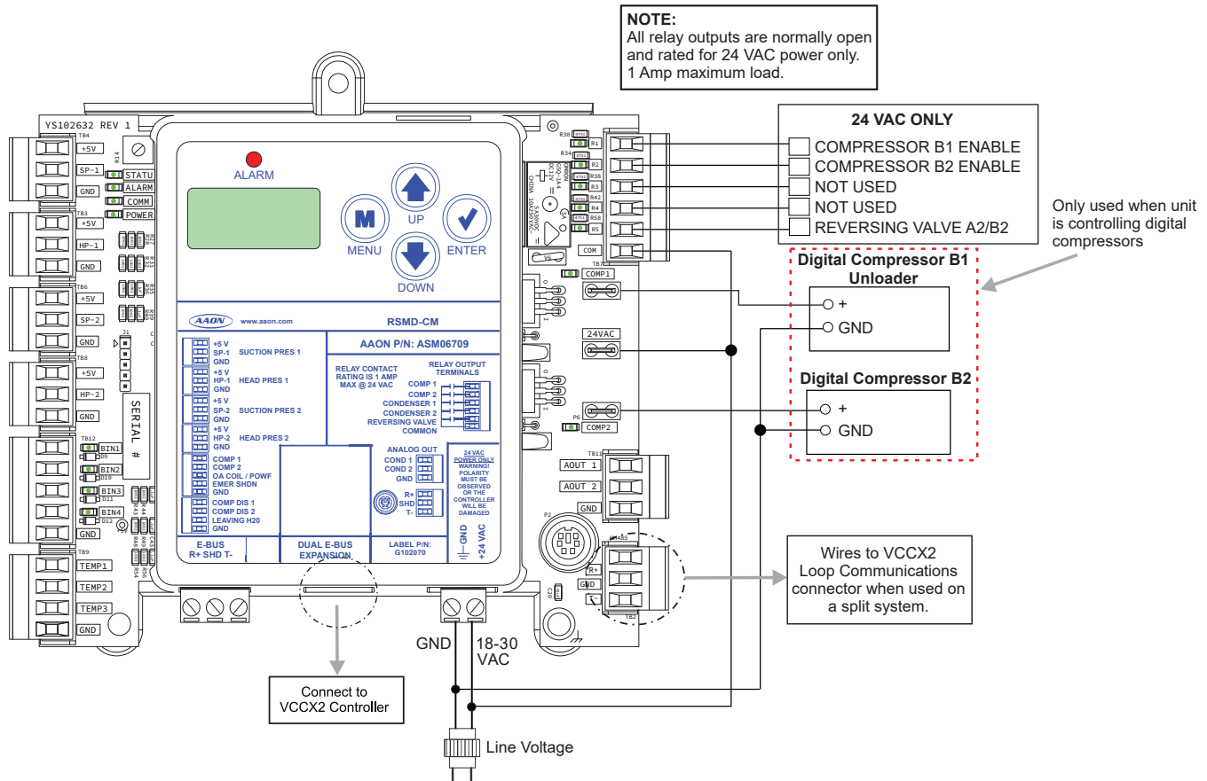
Figure 15: A2/B2 Wiring
