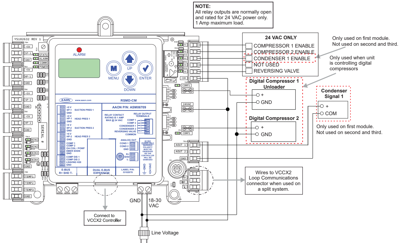
Figure 12: Single Condenser for Three Modules
