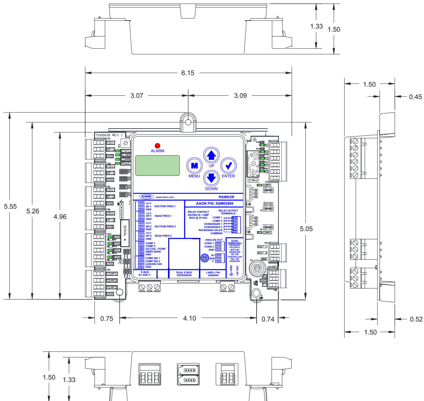
Figure 1: RSMD2R Dimensions
