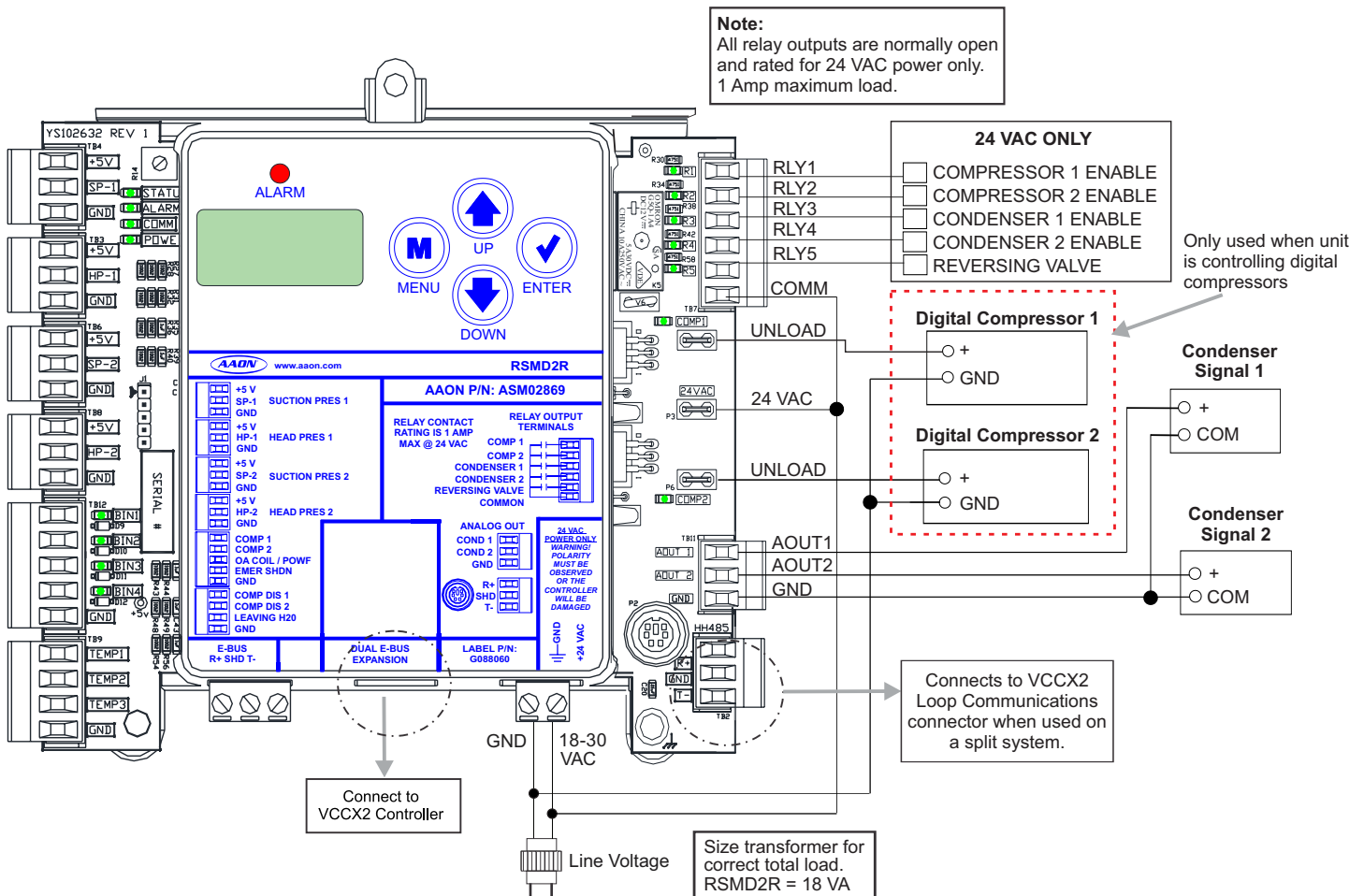
Figure 8: Single Condenser Per RSMD2R Module Wiring
