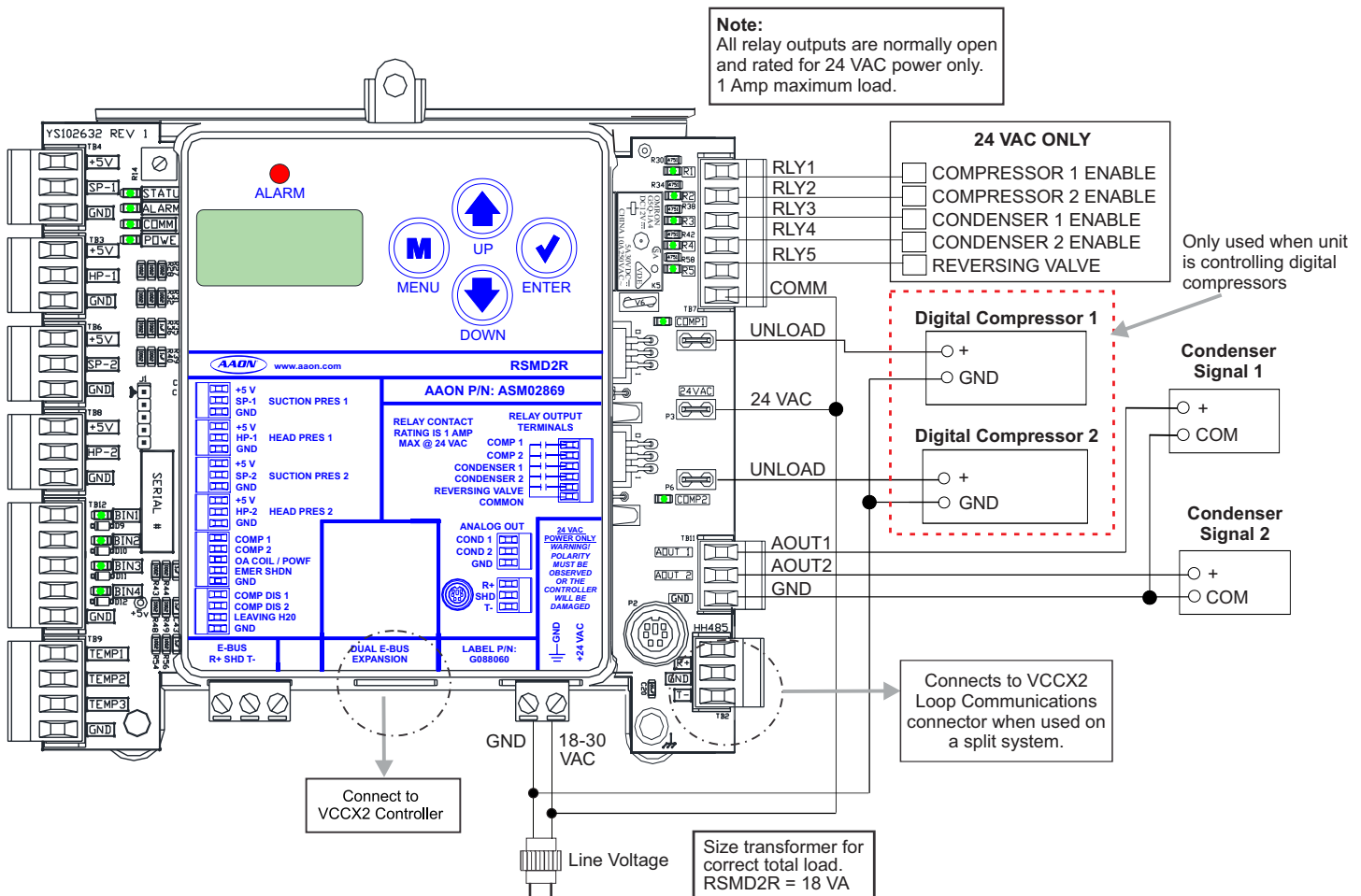
Figure 6: Default: Two Condenser RSMD2R Module Wiring
