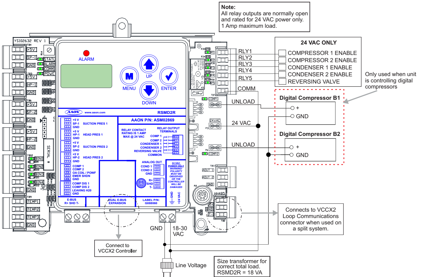
Figure 15: A2/B2 Wiring
