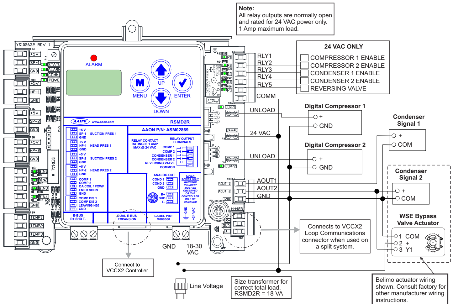
Figure 3: RSMD2R Outputs Wiring
