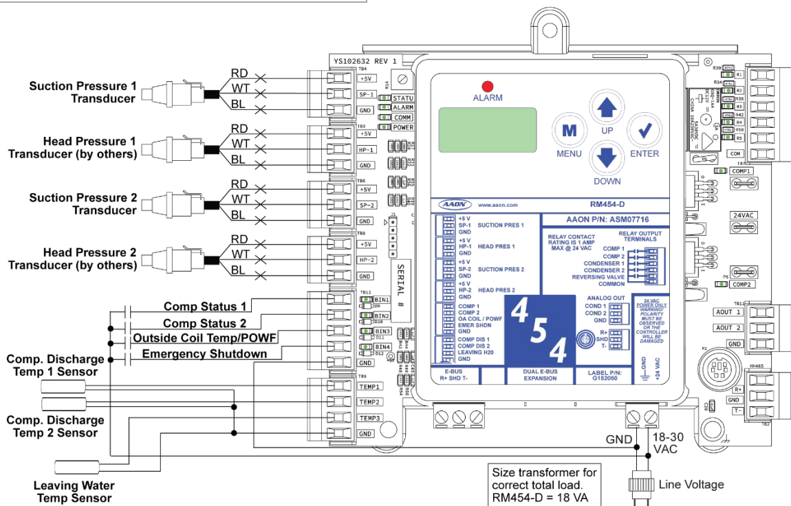
Figure 2: RM454-D Inputs Wiring
