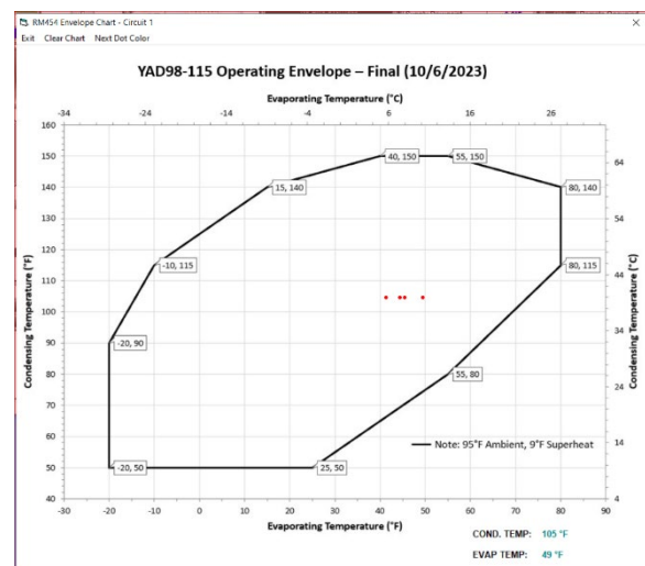
Figure 7: Copeland YAD98-115 Envelope
