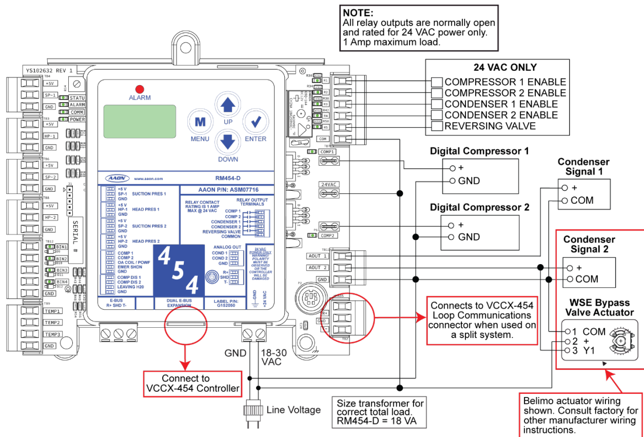
Figure 3: RM454-D Outputs Wiring
