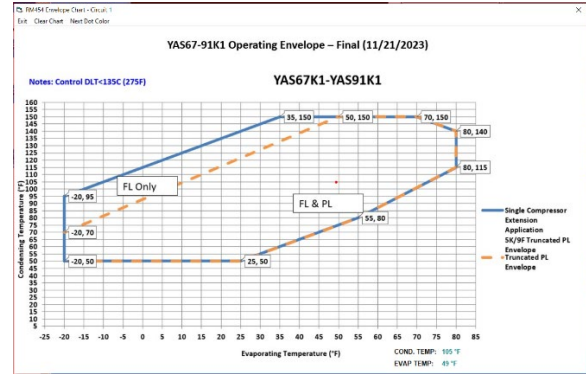
Figure 6: Copeland YAS67K1-91K1 and R454 Envelope
