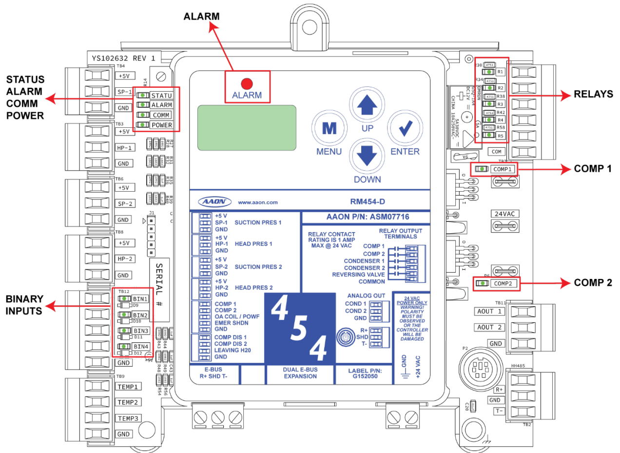
Figure 12: RM454-D LED Locations
