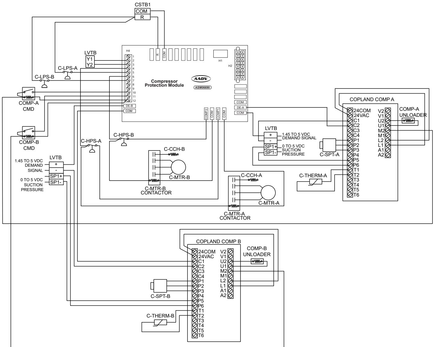
Figure 7: ASM06690 - Dual Digital Compressors
