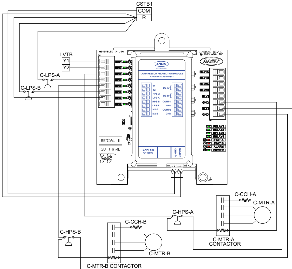
Figure 9: ASM07681 - Dual Compressor
