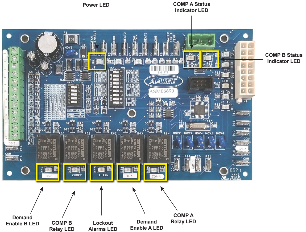
Figure 14: LED Locations and Descriptions - ASM06690
