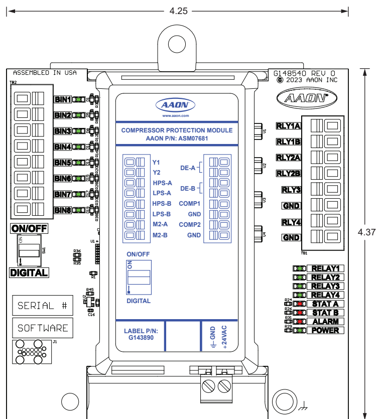
Figure 1: Compressor Protection Module Dimensions - ASM06690
