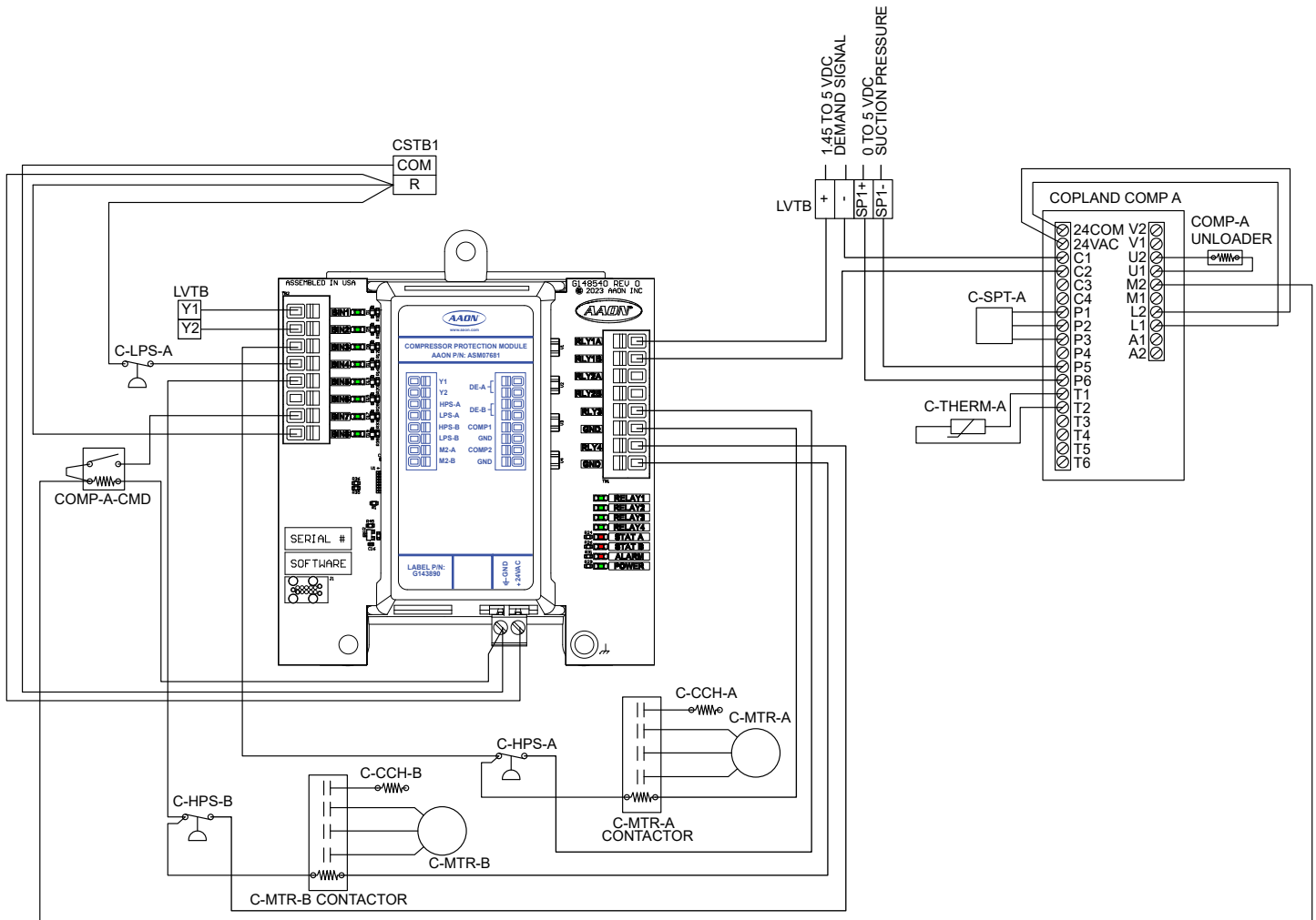
Figure 11: ASM07681 - Digital and On/Off Compressor
