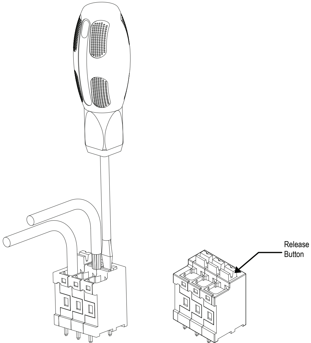
Figure 13: OMNIMATE Connector Instructions
