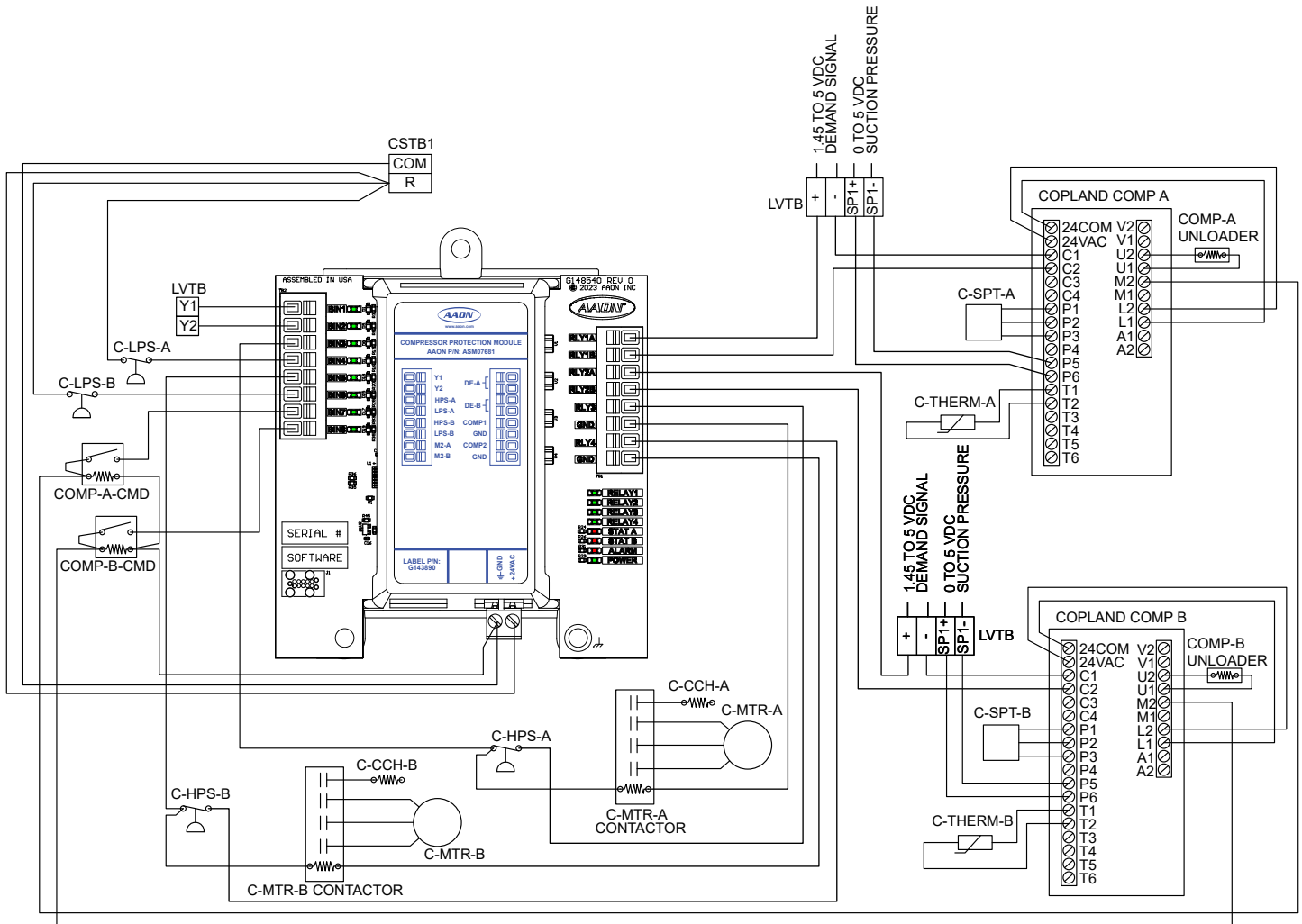
Figure 12: ASM07681 - Dual Digital Compressors
