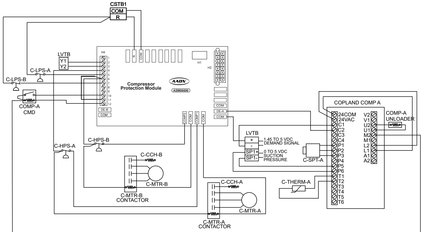
Figure 6: ASM06690 - Digital and On/Off Compressor
