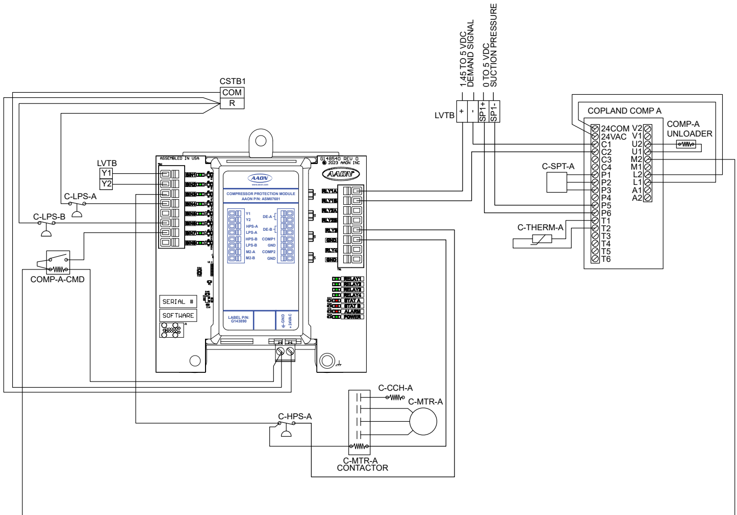
Figure 10: ASM07681 - Single Digital Compressor
