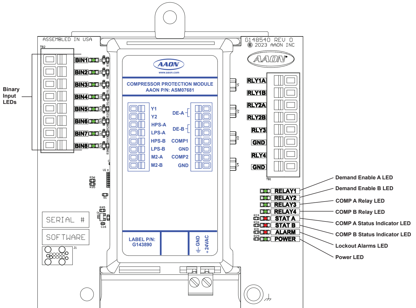
Figure 15: LED Locations and Descriptions - ASM07681
