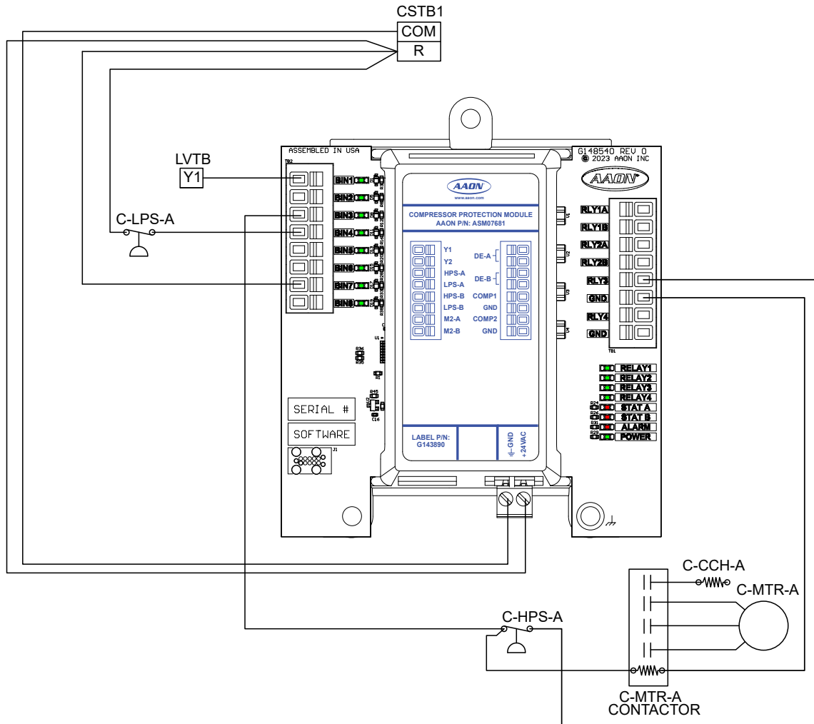
Figure 8: ASM07681 - Single Compressor
