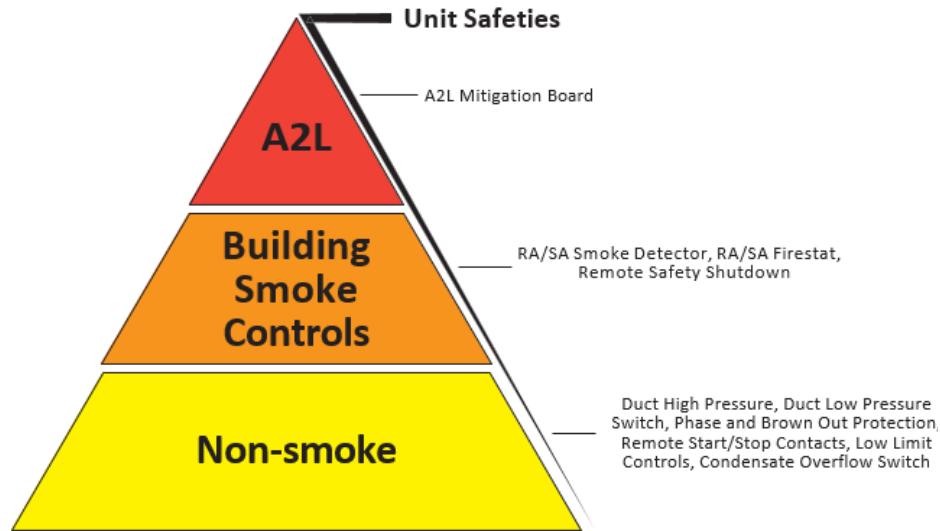
Figure 42: Unit Safety Hierarchy
