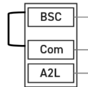
Figure 44: Building Smoke Control Priority Jumper
