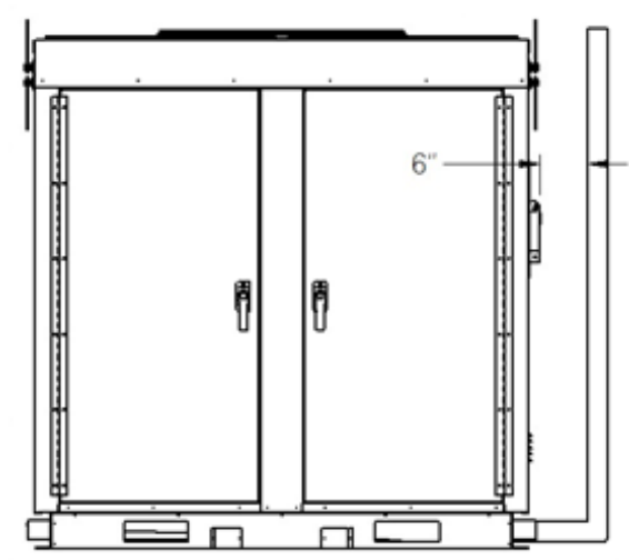
Figure 2: Forklifting a CF Series B and C Cabinet
