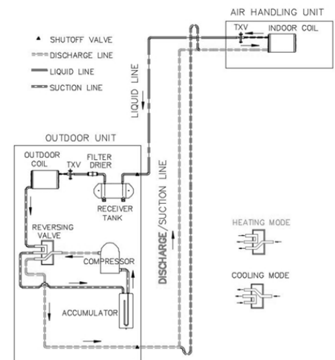
Figure 12: Heat Pump Piping Schematic of Heating Mode in Double Riser
