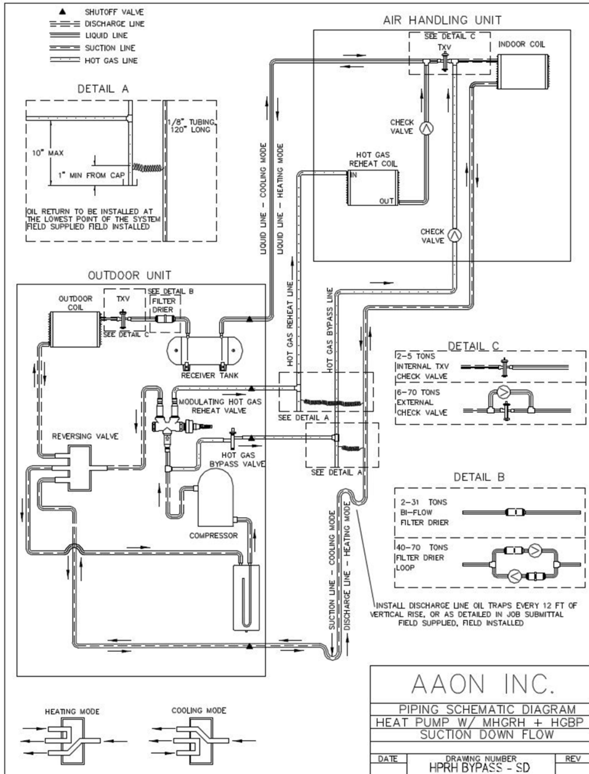
Figure 40: Heat Pump with Modulating Hot Gas Reheat and Hot Gas Bypass Split System Piping, Suction Down
