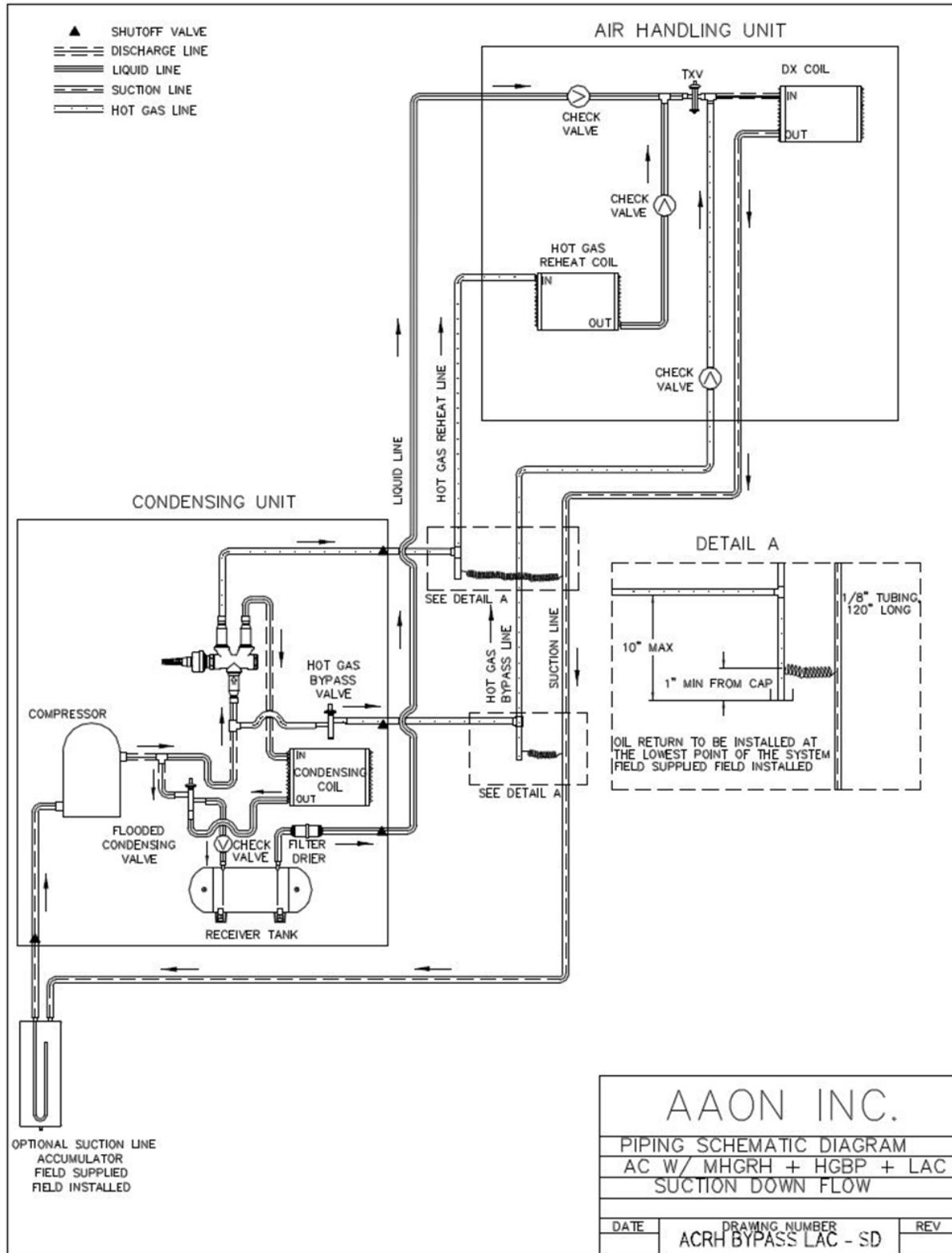
Figure 32: A/C with Modulating Hot Gas Reheat and Hot Gas Bypass + LAC Split System Piping, Suction Down
