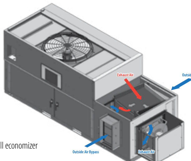
▶ Cross-Flow Fixed Plate Energy Recovery Airflow
