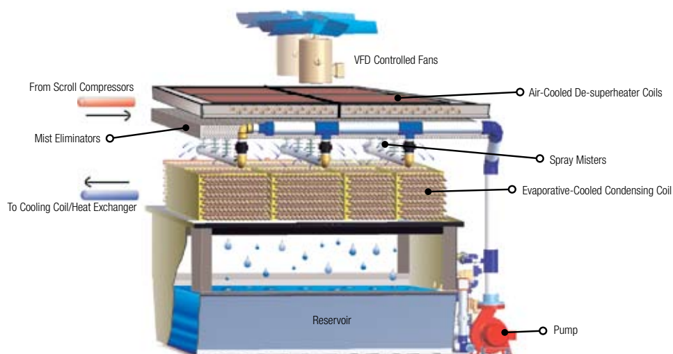
Patented Evaporative-Cooled Condenser
